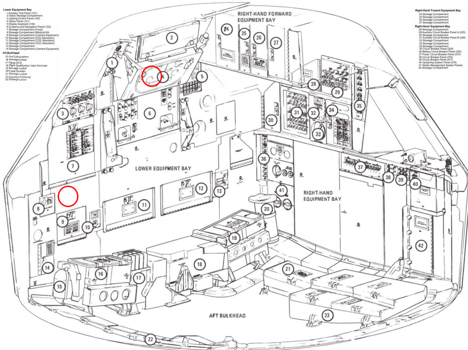
AFT BULKHEAD, LOWER, AND RIGHT-HAND EQUIPMENT BAYS
